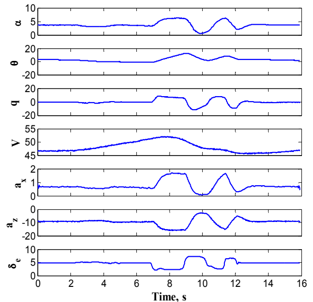
Fig. 2 Real flight data at moderate A.O.A: 3-2-1-1 input
