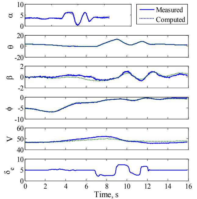
Fig. 4 Measured and computed variables during FPR; 3-2-1-1 input
