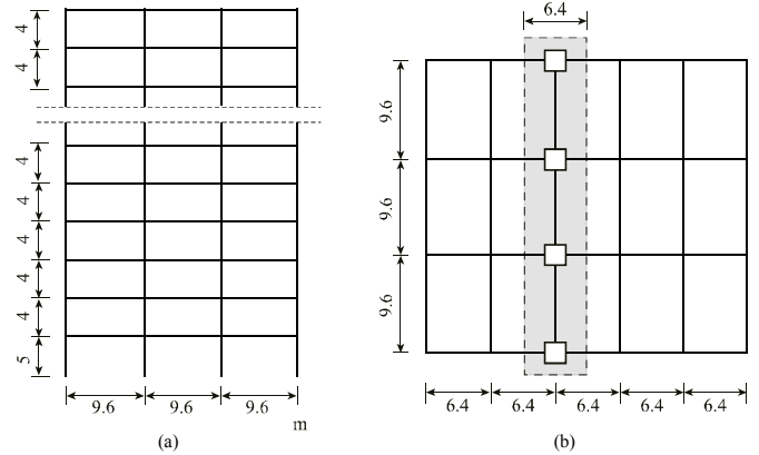
Fig. 1 The SMRF model: (a) elevation and (b) plan
