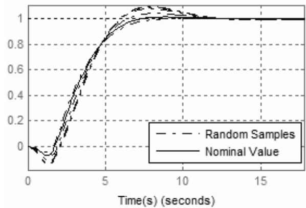
Fig. 10 Robustness of the H_{\infty} controller
