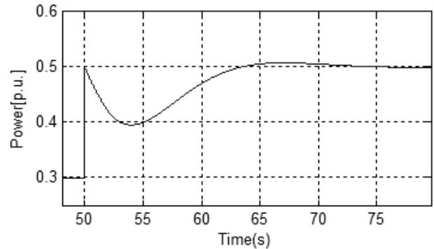
Fig. 9 Active Power with H_{\infty} controller
