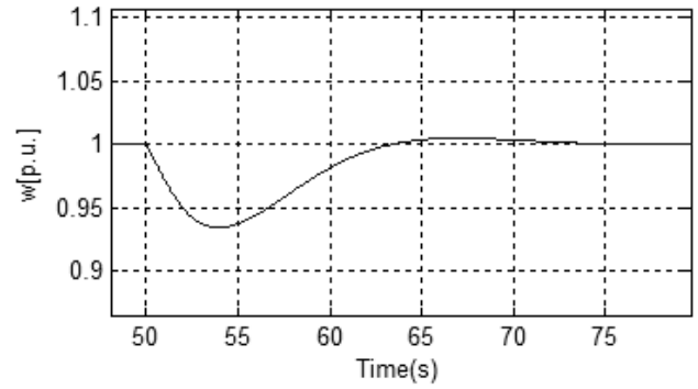
Fig 8 Speed of the turbine with H_{\infty} controller
