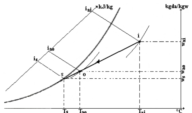
Fig. 1 Psychrometric chart of cooling and dehumidifying process. As a result, both the specific humidity and the local dew point temperature of the leaving air will be lowered. Fig. 1 shows psychrometric chart of cooling and dehumidifying process
