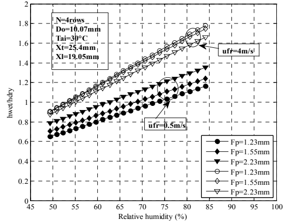
Fig. 3 Effect of inlet relative humidity on h_{wet}/h_{dry}
