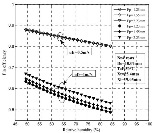
Fig. 2 Variation of fin efficiency with the relative humidity
