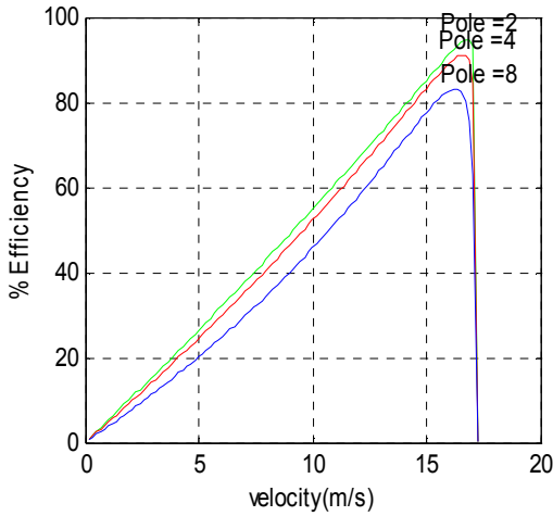
Fig. 9 Effect of number of poles on the efficiency of LIM
