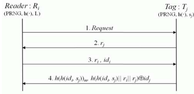
Fig. 3 Authentication protocol proposed by Tan et al.
