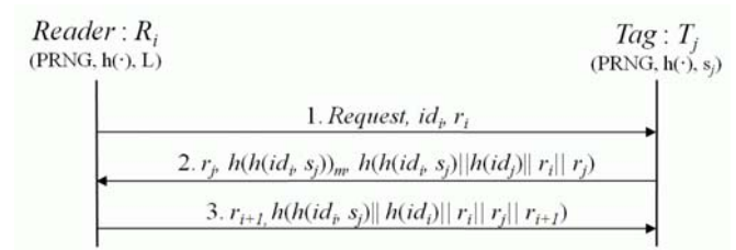
Fig. 5 The proposed protocol
