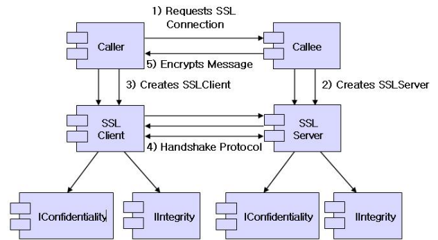
Fig. 3 Transmission of the RMI-based SSL Message
