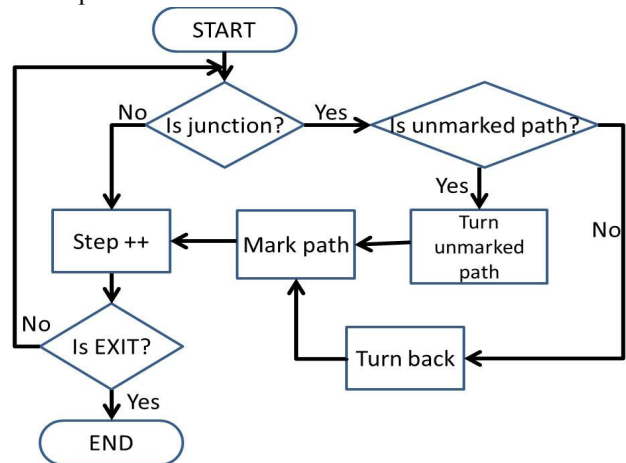
Fig. 2 Tremaux's algorithm [4]
