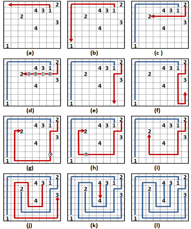
Fig. 4 Solving Number Link with modified Tremaux's Algorithm
