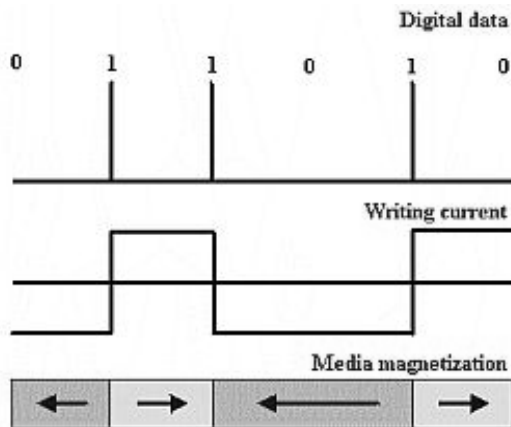
Fig. 2 TheMagnetic Recording Basics.
