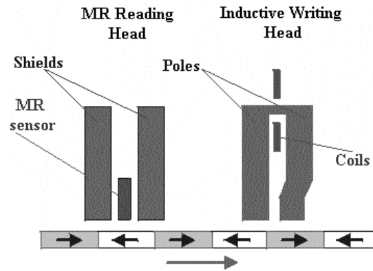
Fig. 3 The MR read/write operating on the media.
