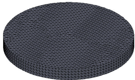
Fig. 2 Discretization of the piezoelectric transformer
