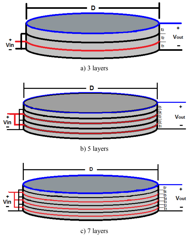
Fig. 1 Detail of the multi-layer piezoelectric transformers
