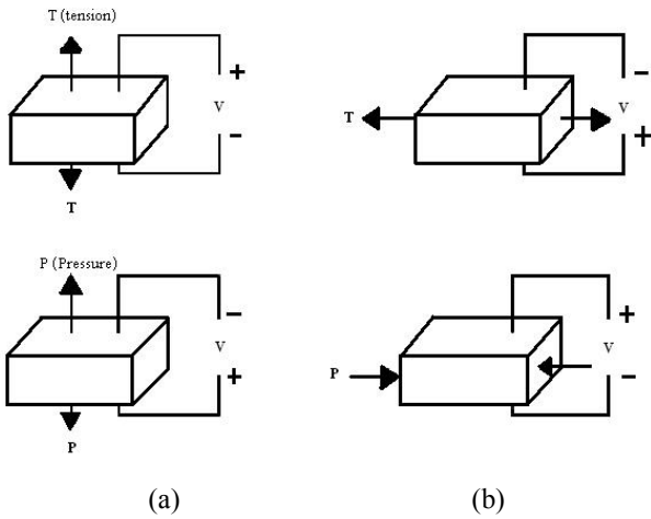
Fig. 1 Piezoelectric effects: (a) longitudinal effects; (b) transverse effects [10]
