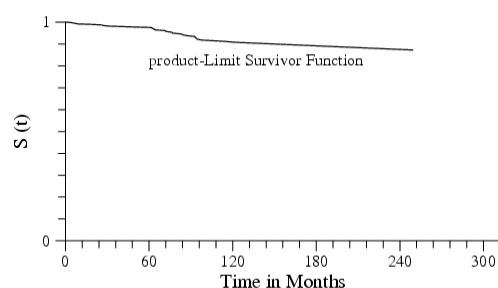
Fig. 1 Product-limit (Kaplan-Meier) survivor function
