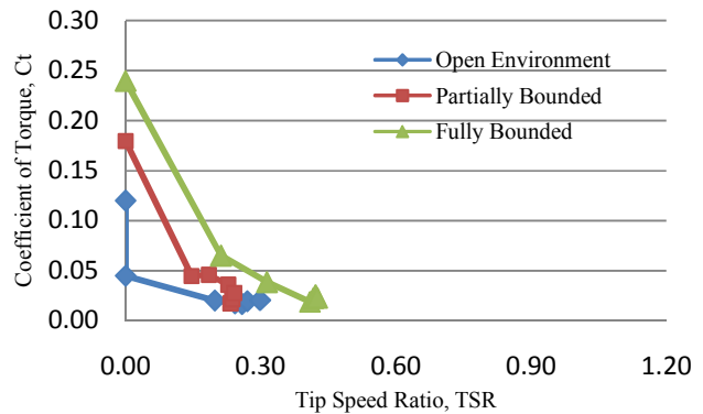
Fig. 15 C_T Results for Rotor 3 at different Operating Environments
