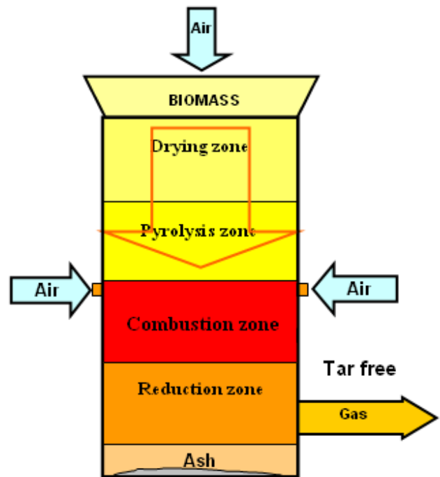
Fig. 2 Shows process zone for downdraft gasifiers
