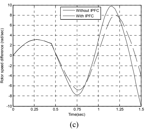
Fig. 7 Variation of generator – 3(6 bus system) rotor speed difference without and with IPFC for different fault clearing times( t_c ), (a) t_c = 0.4 (b) t_c = 0.5 (c) t_c = 0.45
