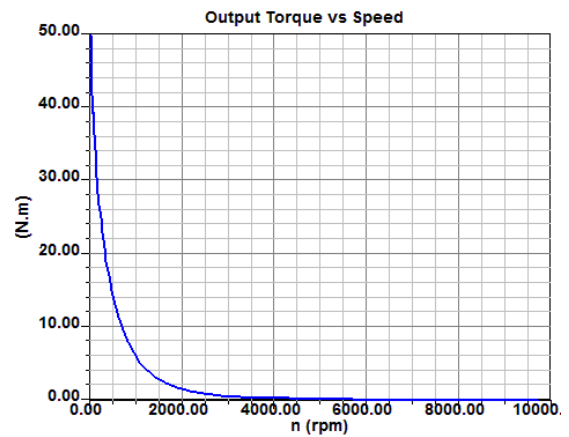
Fig. 13 torque versus speed
