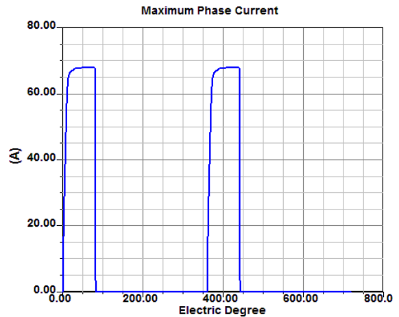
Fig. 14 phase current versus electrical degree
