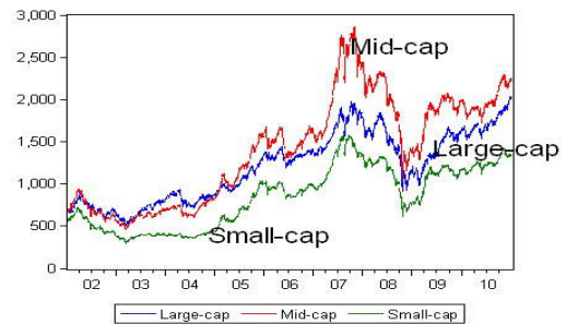
Fig. 1 Daily price indices (January 2, 2002 ~ December 30, 2010)
