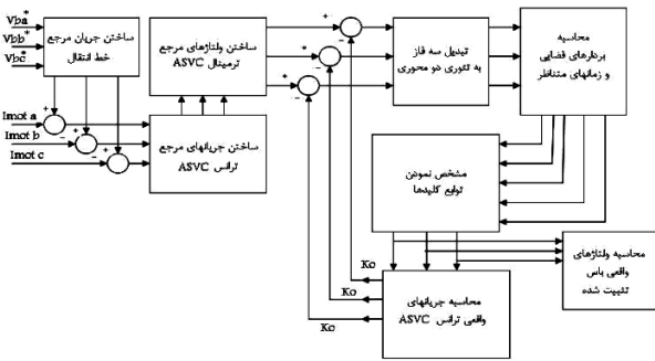
Fig. 4 Diagram block
