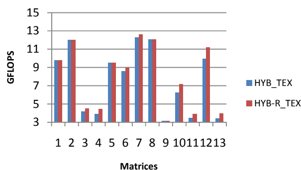
Fig. 5 Single precision performance with cache on GeForce 9800 GX2.
