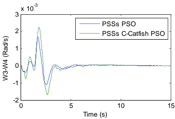
Fig. 6 Inter-area and local mode of oscillations for OP 1
