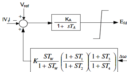
Fig. 3 Block diagram of the AVR equipped with PSS
