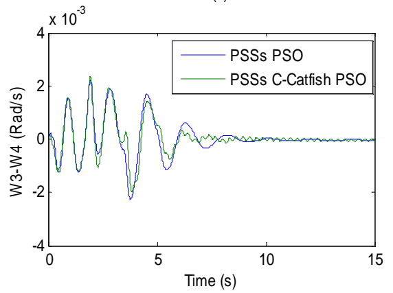
Fig. 7 Inter-area and local mode of oscillations for OP 2
