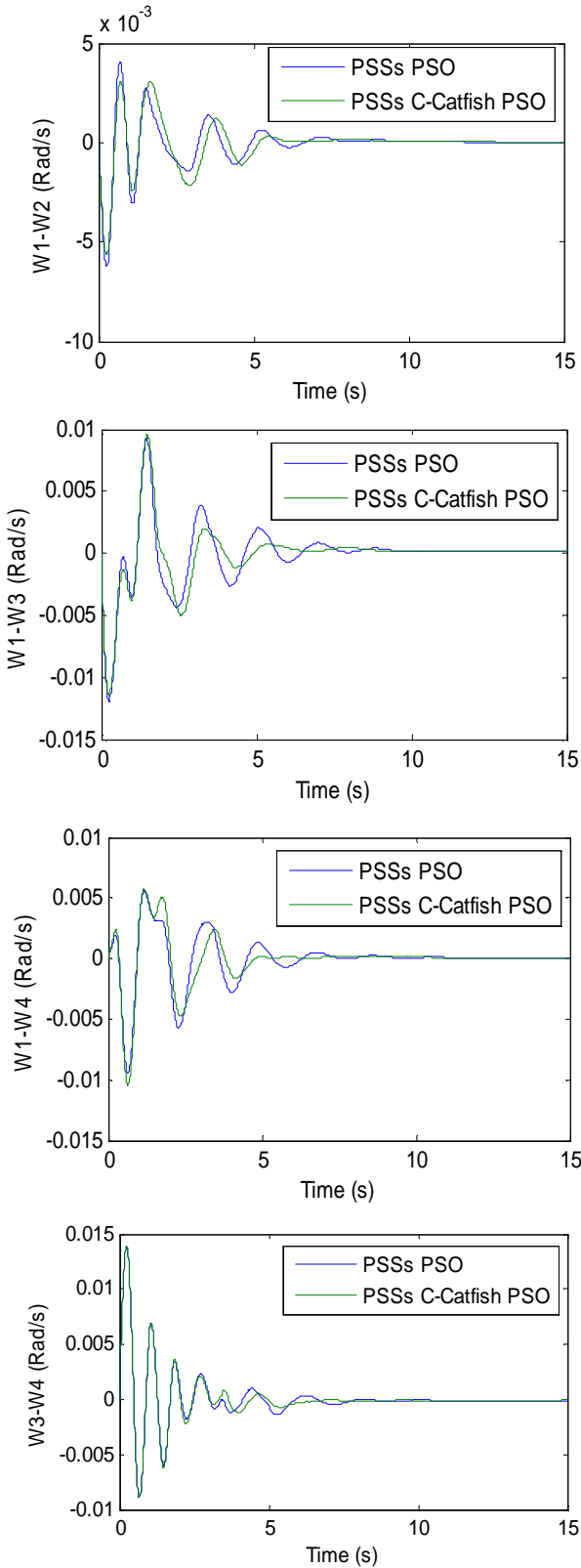
Fig. 8 Inter-area and local mode of oscillations for OP 3
