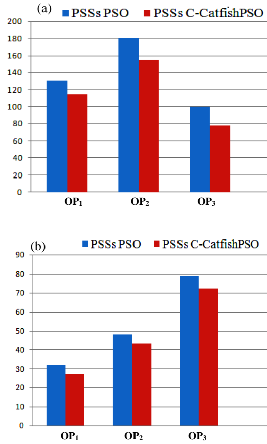
Fig. 9 Values of performance index: (a) FD and (b) ITAE
