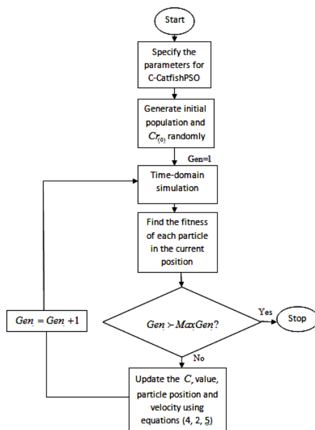
Fig. 1 Flowcharts of C-Catfish PSO algorithm
