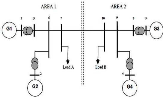
Fig. 2 Multi-machine power system
