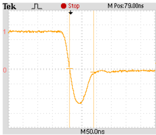
Fig. 9 Experimental reverse recovery waveform at di/dt=100A/\mu s , I_F=1A , V_R=30V , (0.4A/div, 50ns/div)
