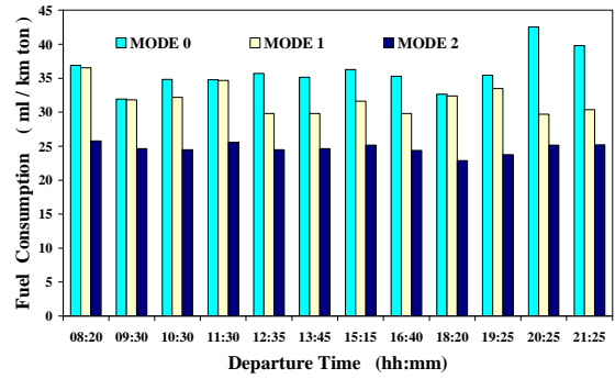
Fig. 10 Fuel consumption variation according to departure time for MODE 0, MODE 1 and MODE 2
