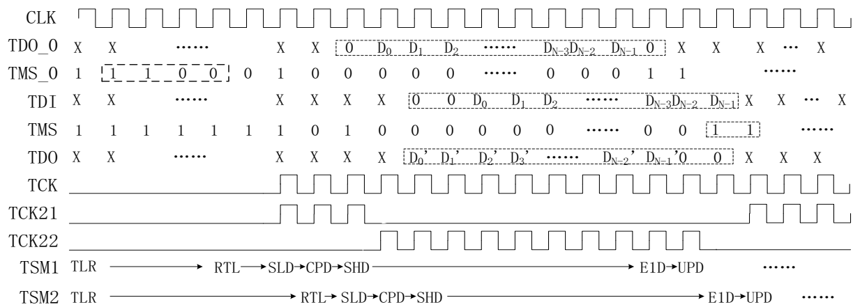
Fig. 10 Timing diagram of this design
