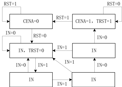
Fig. 8 State diagram of the RSC
