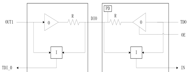
Fig. 9 Architecture of the SBT circuit
