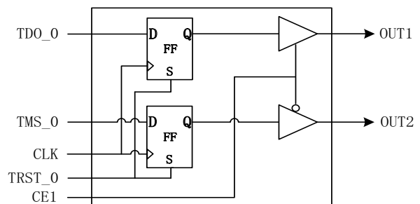
Fig. 4 Architecture of the DSC
