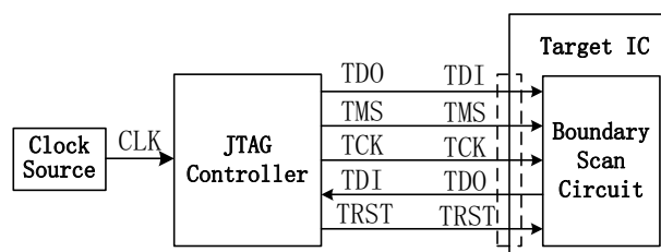
Fig. 1 A conventional 5-signal interface circuit
