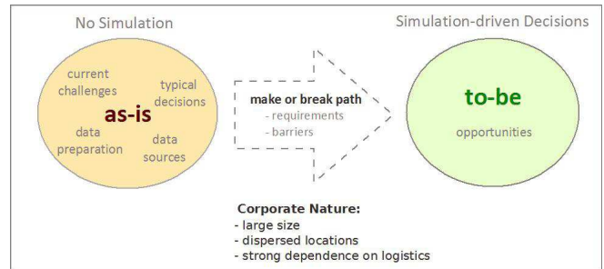
Fig. 2 Research Framework
