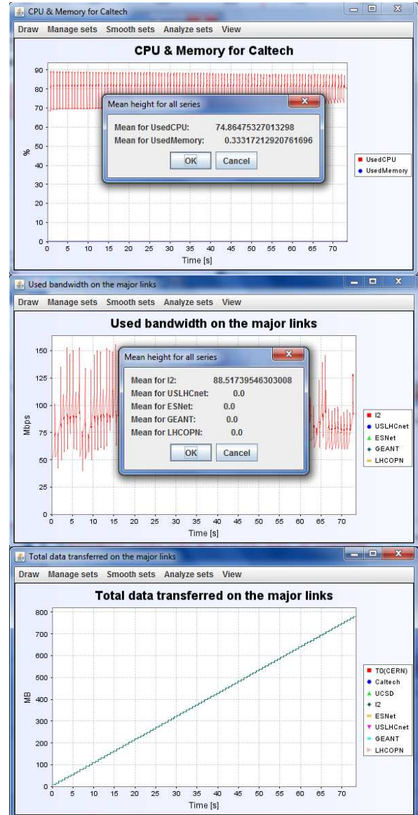
Fig. 4 Validation results showing the average CPU load at Caltech, the throughput, and the total data transferred
