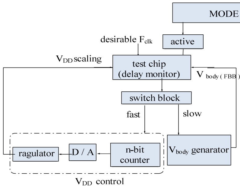
Fig. 1 Diagram of proposed design for active mode
