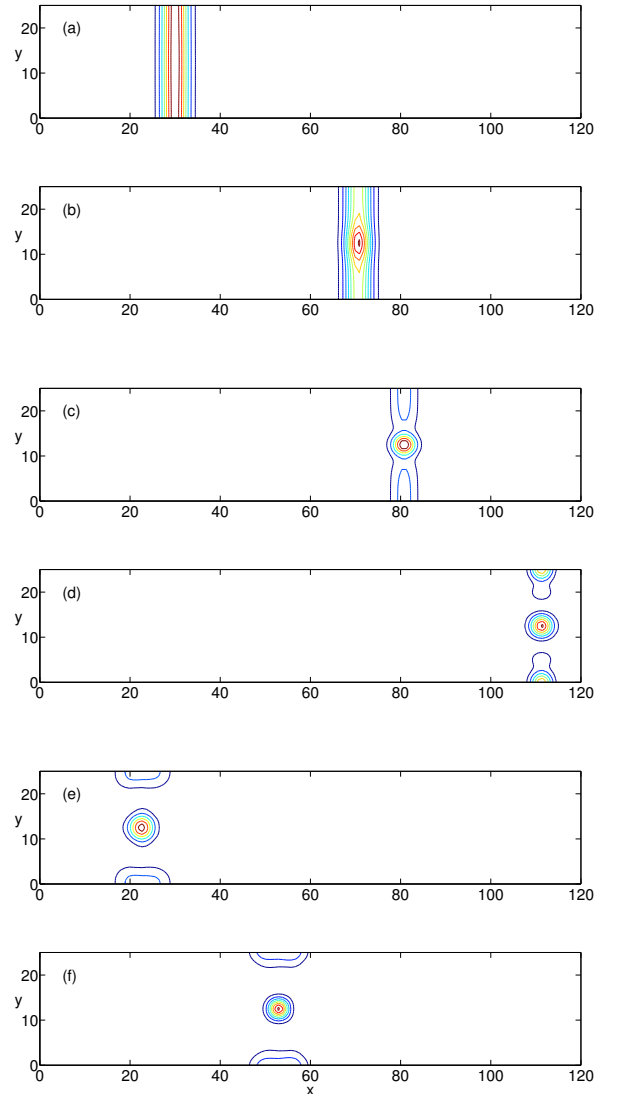
Fig. 2. Contour plot of |\phi| showing the time evolution of a perturbed plane soliton with V = 2.0 , \eta = 0.25 : (a) t = 0.0 , (b) t = 0.002 , (c) t = 0.0025 , (d) t = 0.004 , (e) t = 0.0175 , (f) t = 0.019 .
