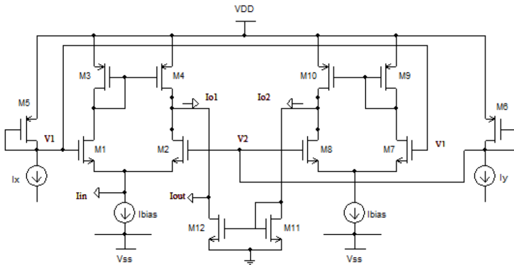
Fig. 2 Complete circuit diagram of proposed design
