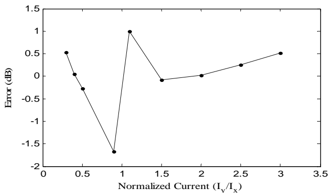
Fig. 4 Errors between the simulated and the theoretical results (@ I_m = 100 nA )
