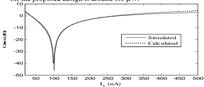
Fig. 3 Simulation results of the proposed VGA ( I_x = 100 nA , I_m = 100 nA )
