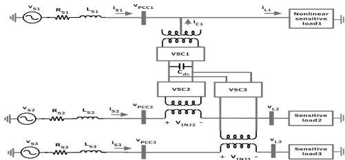
Fig. 2 Shunt and series compensators of GUPQC
