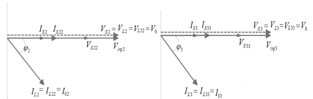
Fig. 7 Phasor representation of series compensators loading
