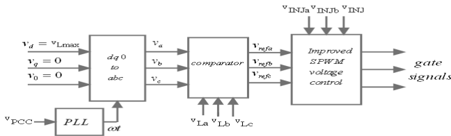
Fig. 5 Series compensator control
