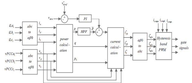
Fig. 4 Shunt compensator control
