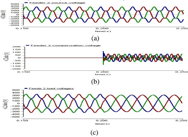
Fig. 9 Feeder2 voltages: (a) supply (b) compensation (c) load
