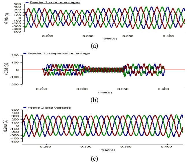
Fig. 11 Feeder2 voltages: (a) supply (b) compensation (c) load
