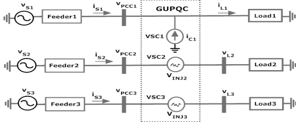
Fig. 1 Distribution system with the proposed GUPQC
