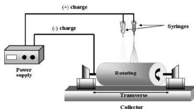
Fig. 1 Schematic diagram of the double-spinneret electrospinning
