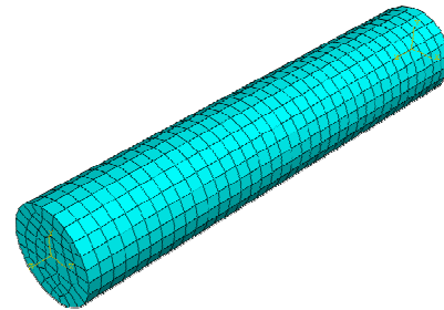
Fig. 5 Typical finite element model of the ceramic rod
