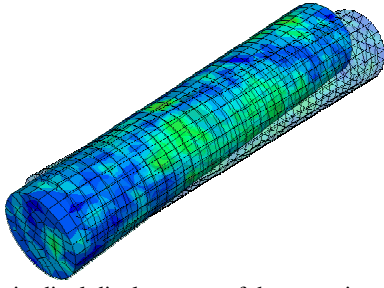
Fig. 6 Longitudinal displacement of the ceramic rod by finite element analysis
