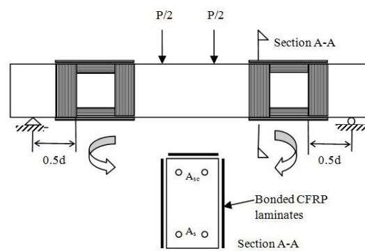
Fig. 2 CFRP strengthening configurations
