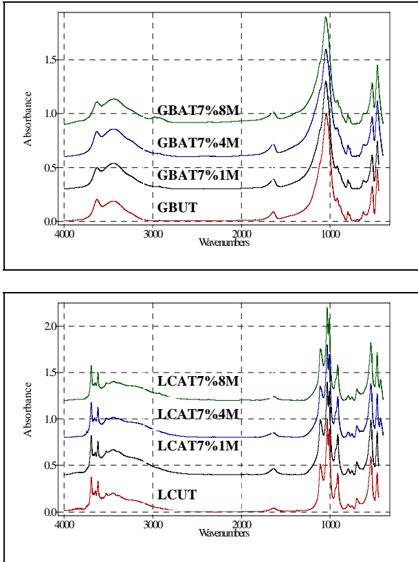
Fig. 1 FTIR of natural and 1, 4, and 8 months cured samples.
