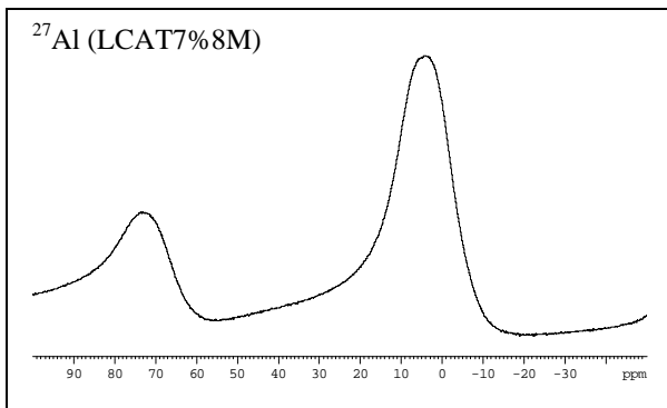
Fig. 2 27 Al MAS NMR spectra of 8 months cured Green Bentonite (GB) and Laterite Clay (LC).
