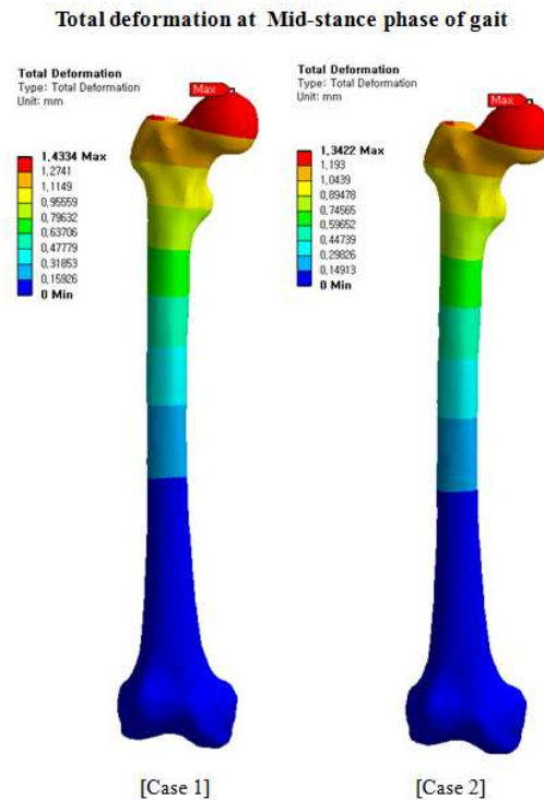
Fig. 6 Contour image of the Total deformation at Case1 & Case2
