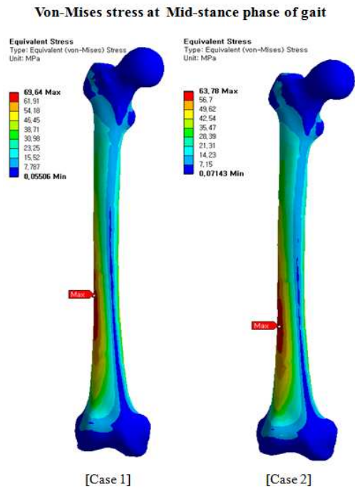
Fig. 5 Contour image of the Von-Mises stress (Maximum Von-Mises stress point (Red tag) of Case1 was different with Case2)
