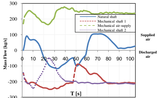
Fig. 5 Mass flow rates at the exits of the shafts when the train runs in the track 2
