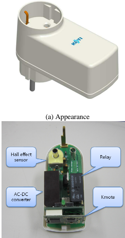
(b) Configuration Fig. 2 Wireless plug
