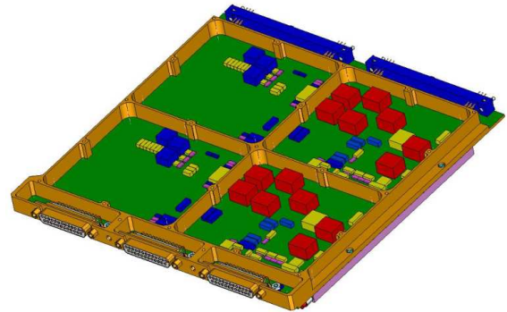
Fig. 5 MPPU electronics boards layout (courtesy of Thales Alenia Space Italia)
