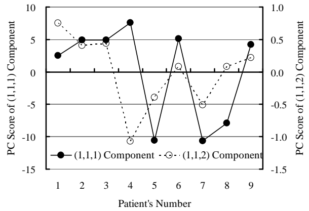
Fig. 6 TPCA scores of (1,1,1) and (1,1,2) components.
