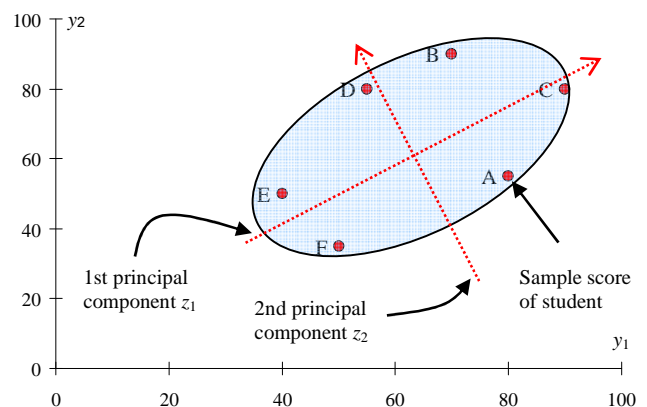
Fig. 1 Conception of the PCA
