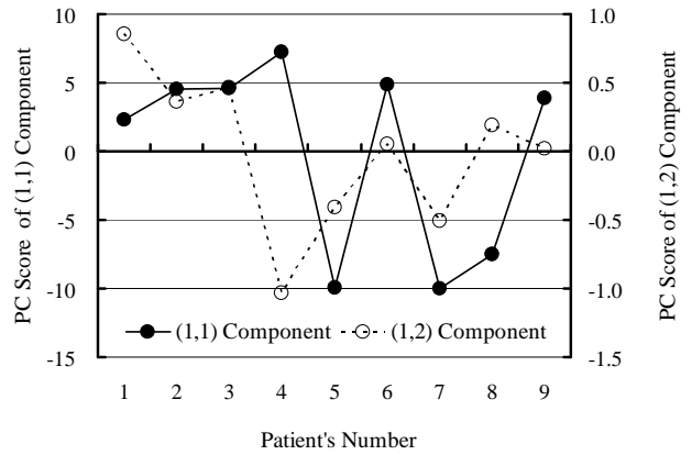
Fig. 3 MPCA scores of (1,1) and (1,2) components.
