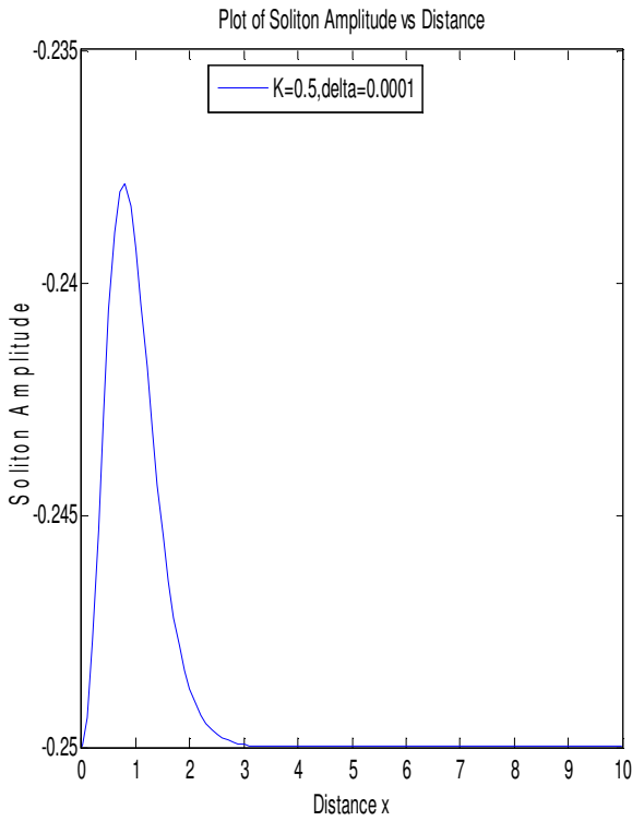
Fig. 1. Plot of Soliton Amplitude vs Distance
