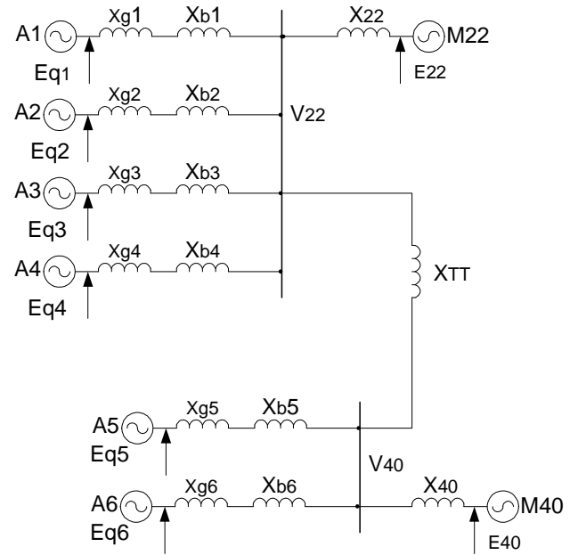
Fig. 3 Simplified internal equivalent single line diagram of the steam power plant "Nikola Tesla A"
