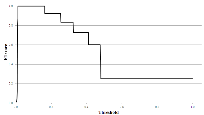
Fig. 8 The dependency of F1 score to threshold for shot cut detection using MSE
