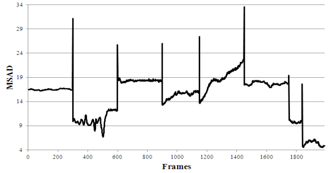
Fig. 3 Plot of cut detection using MSAD for proposed method
