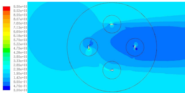
Fig. 13 Contours of absolute velocity [m/s] for the whole rotor for the angular position of maximum torque coefficient ( \theta= 92^\circ ), N=4 , \lambda=2.43
