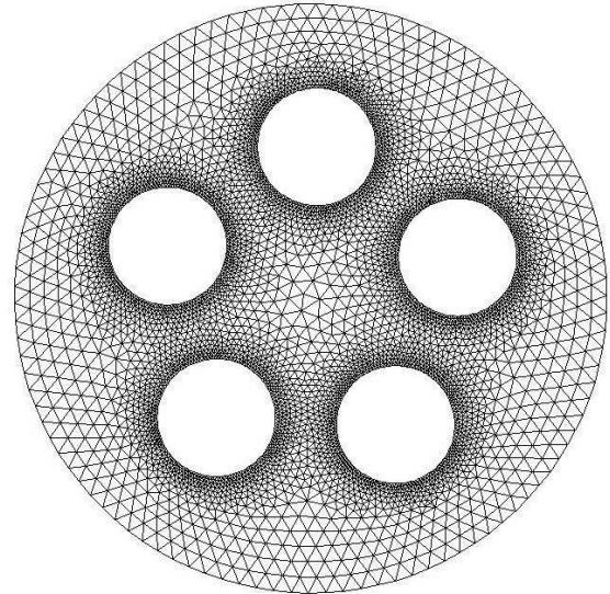
Fig. 4 Rotor sub-grid mesh for the five-bladed VAWaterT architecture
