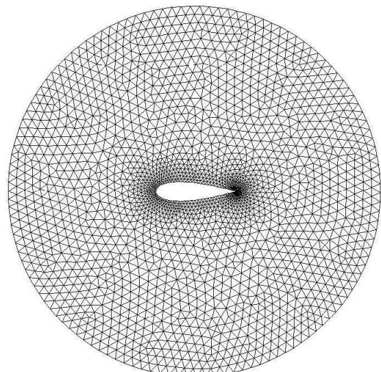
Fig. 5 Control circle grid for NACA 0025 blade section
