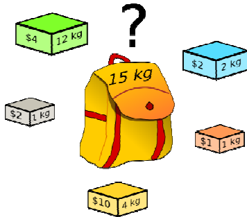
Fig. 1 Knapsack supplier
