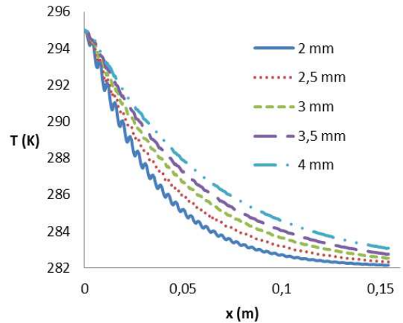
Fig. 11 temperature development along the sinusoidal fins
