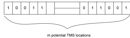
Fig. 7 Solution representation
