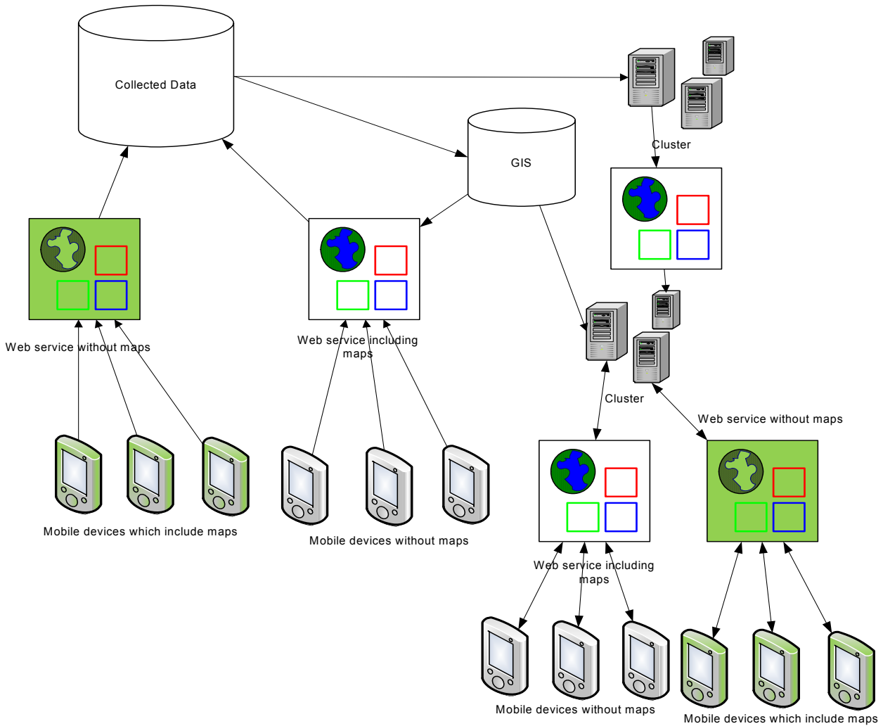
Fig. 1. System architecture
