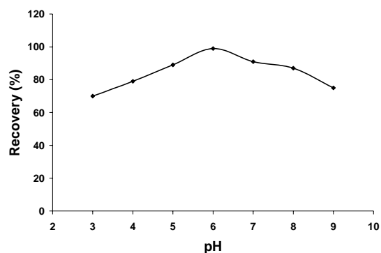
Fig. 3 Effect of pH sorption of Cu (II) onto 1-amino-2-naphthol – Amberlite XAD-4.
