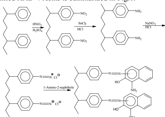
Fig. 1. The methodology of synthesise of 1-amino-2-naphthole – Amberlite XAD-4.
