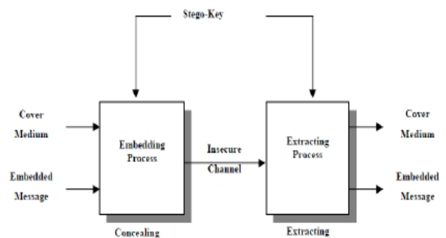
Fig. 1. Steganographic Process
