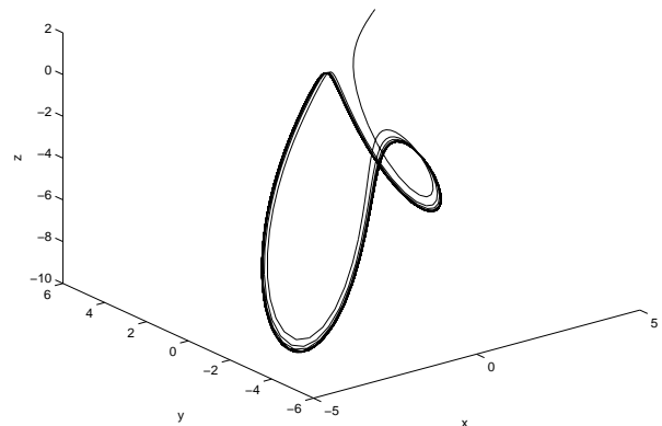
Fig. 3. Phase diagram of system (3) with a = -5, b = 5, c = -4 and d = -3 .
