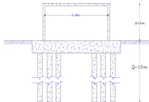
Fig. 1 frame of a building constructed on pile
