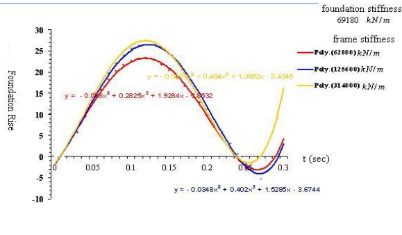
Fig. 4 the effect of frame stiffness on foundation transformation
